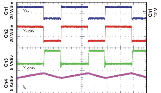
CONTINUOUS CONDUCTION MODE (CCM) SWITCHING WAVEFORMS
