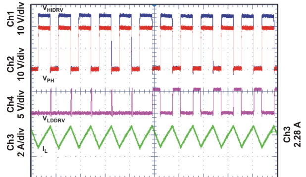
NONSYNCHRONOUS TO SYNCHRONOUS TRANSITION
